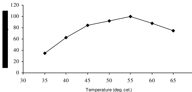
Fig 1: Relative Anti-Pilling Score of PISCEAN R2333L at pH 4.5
