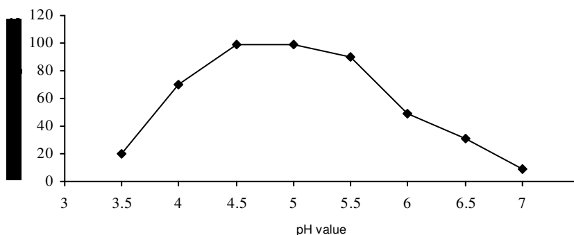
Fig 2: Relative Anti-Pilling Score of PISCAN R2333L at 55 deg. cel.
