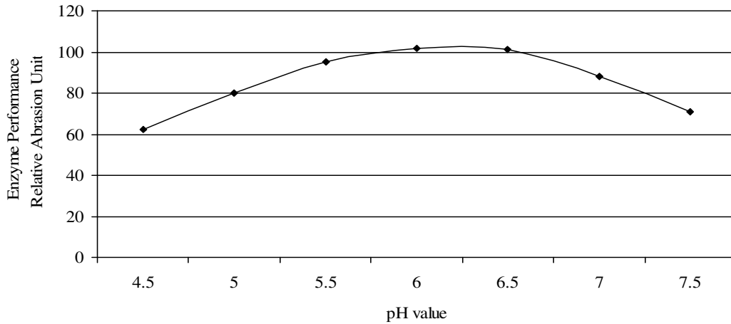
Fig.2 Relative Abrasion Units of Piscean MGC against variable pH at 40 deg. Cel.
