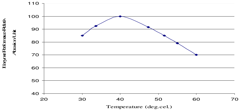
Fig.1 Relative Abrasion Units of PISCEAN EE757I against variable temperature range at pH5.5
