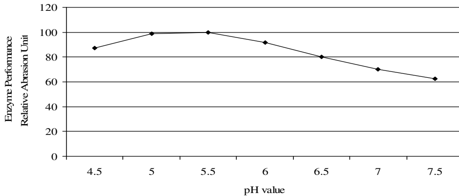
Fig.2 Relative Abrasion Units of PISCEAN EE757I against variable pH at 40 deg. Cel.
