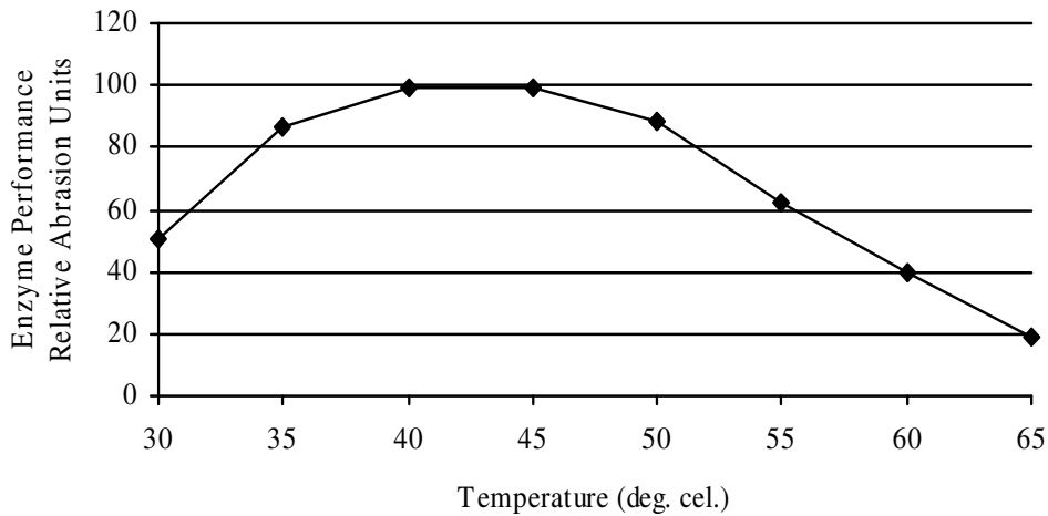
Fig.1 Relative Abrasion Units of PISCEAN BTS-75F against variable temperature range at pH 6.0
